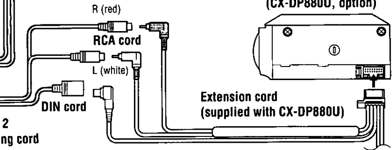
CD changer (CX-DP880U, option)
